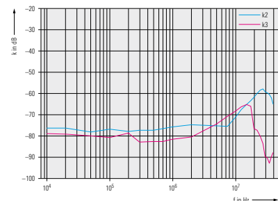
Low harmonics of the analog I/Q outputs of the R&S® AMU200A
